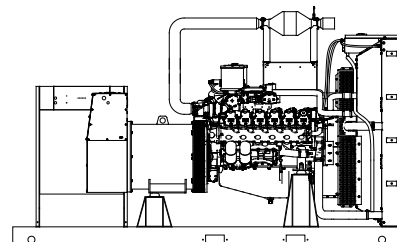
“OPEN” GEN-SET
